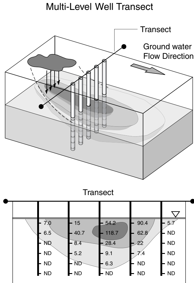
FIGURE 11.4 Transect of multilevel wells. (Illustration courtesy of LFR Levine–Fricke and the American Petroleum Institute.)
