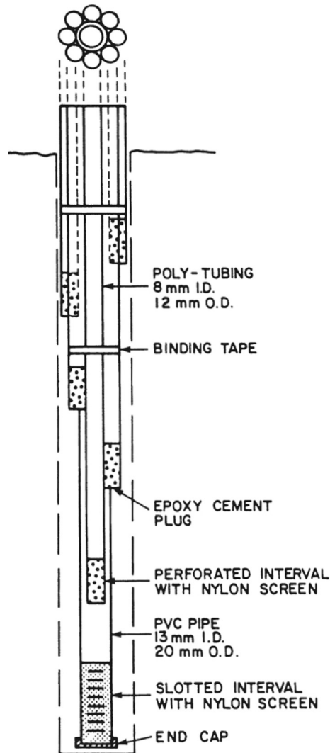
FIGURE 11.7 Bundle well. (From Cherry et al. [1983]. With permission.)
