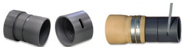
O-Ring Joints with Shear Wire
