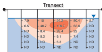
Multilevels Provide Three Dimensional Groundwater Data. Illustration courtesy of LFR Levine-Fricke and the American Petroleum Institute
